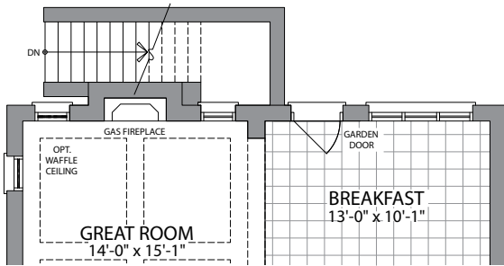
GROUND FLOOR W/OPT. BASEMENT SECONDARY SUITE ELEVATION A & B
