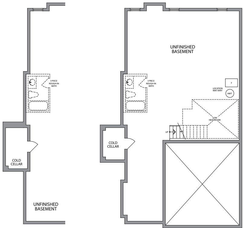
BASEMENT ELEVATION B
