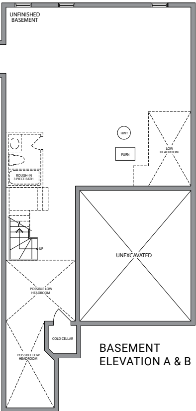
OPT. BASEMENT W/SECONDARY SUITE ELEVATION A & B
