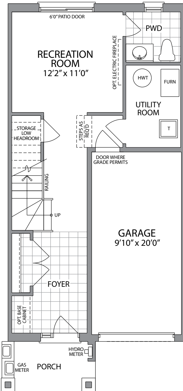
LOWER FLOOR ELEVATION A
