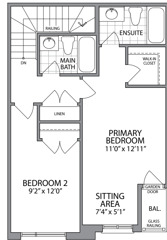
OPT. UPPER FLOOR 2 BEDROOM ELEVATION A
