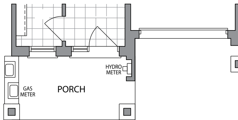
LOWER FLOOR ELEVATION B
