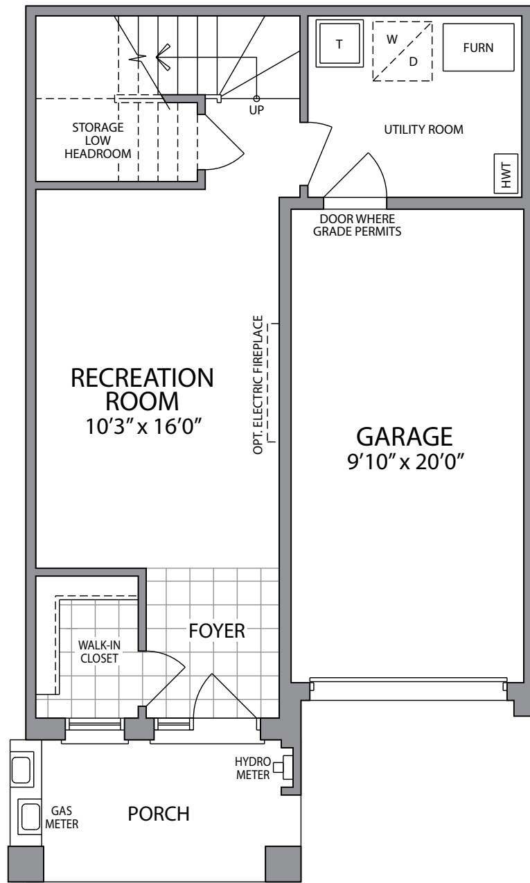
LOWER FLOOR ELEVATION A
