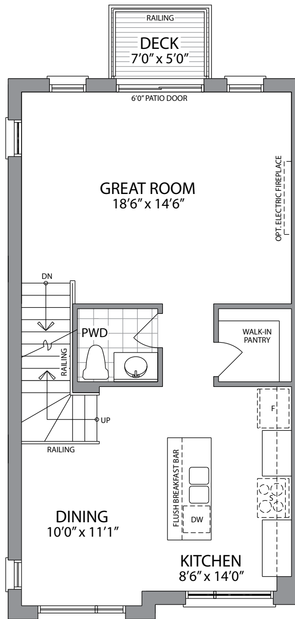
MAIN FLOOR ELEVATION A
