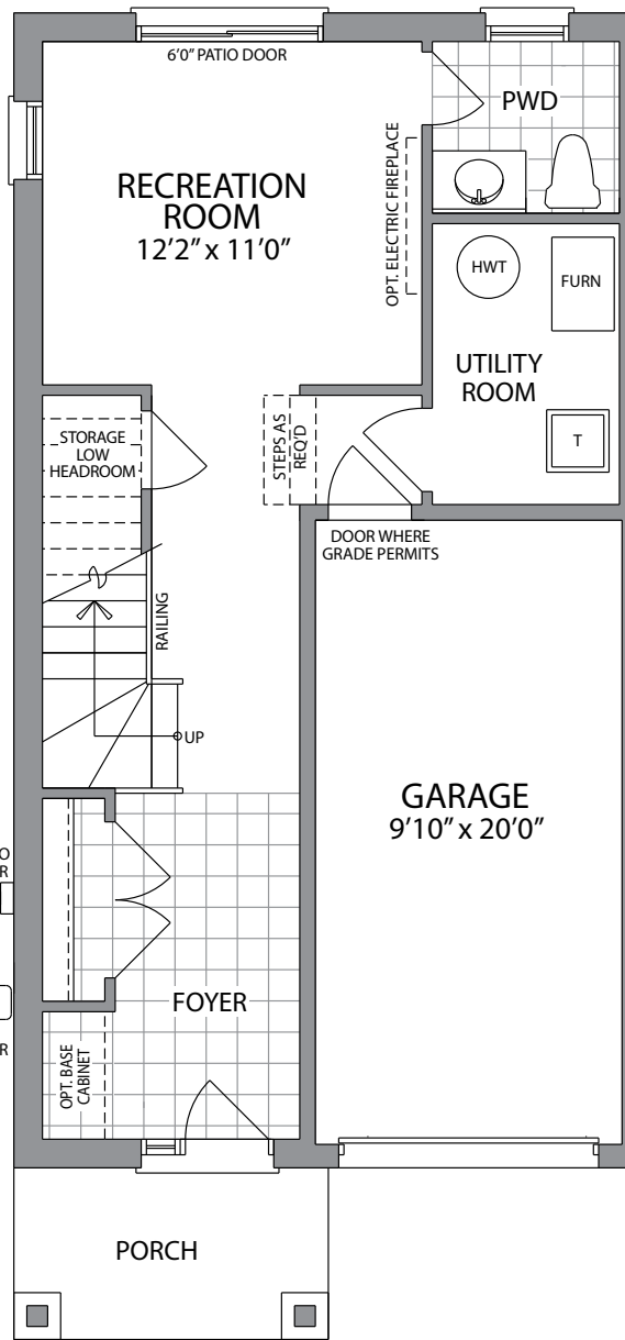
LOWER FLOOR ELEVATION A
