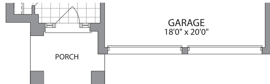
GROUND FLOOR ELEVATION B
