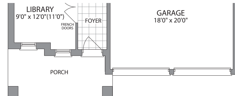
GROUND FLOOR ELEVATION B
